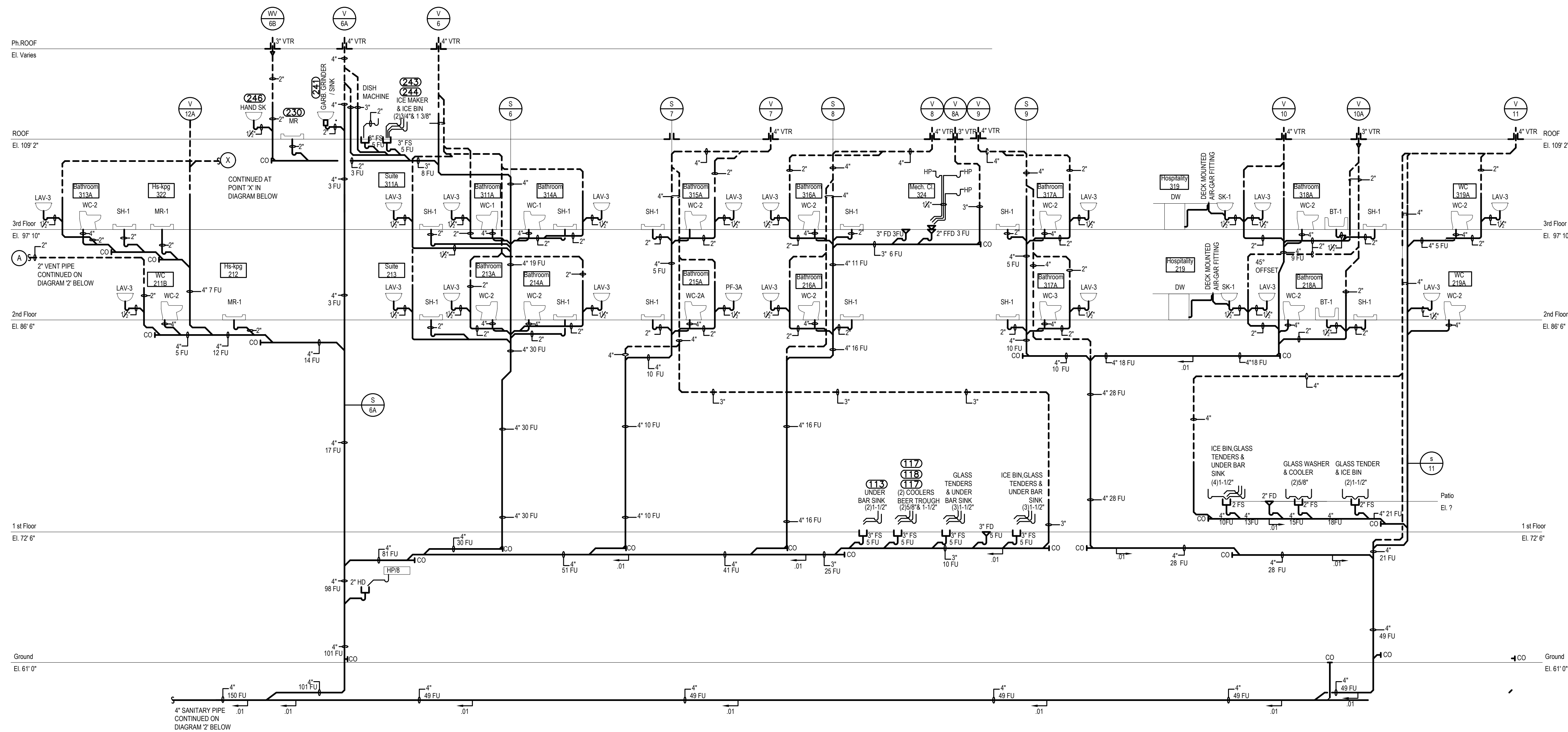
1 PARTIAL SANITARY RISER DIAGRAM PART - 'A' P-7 SCALE : NO SCALE
