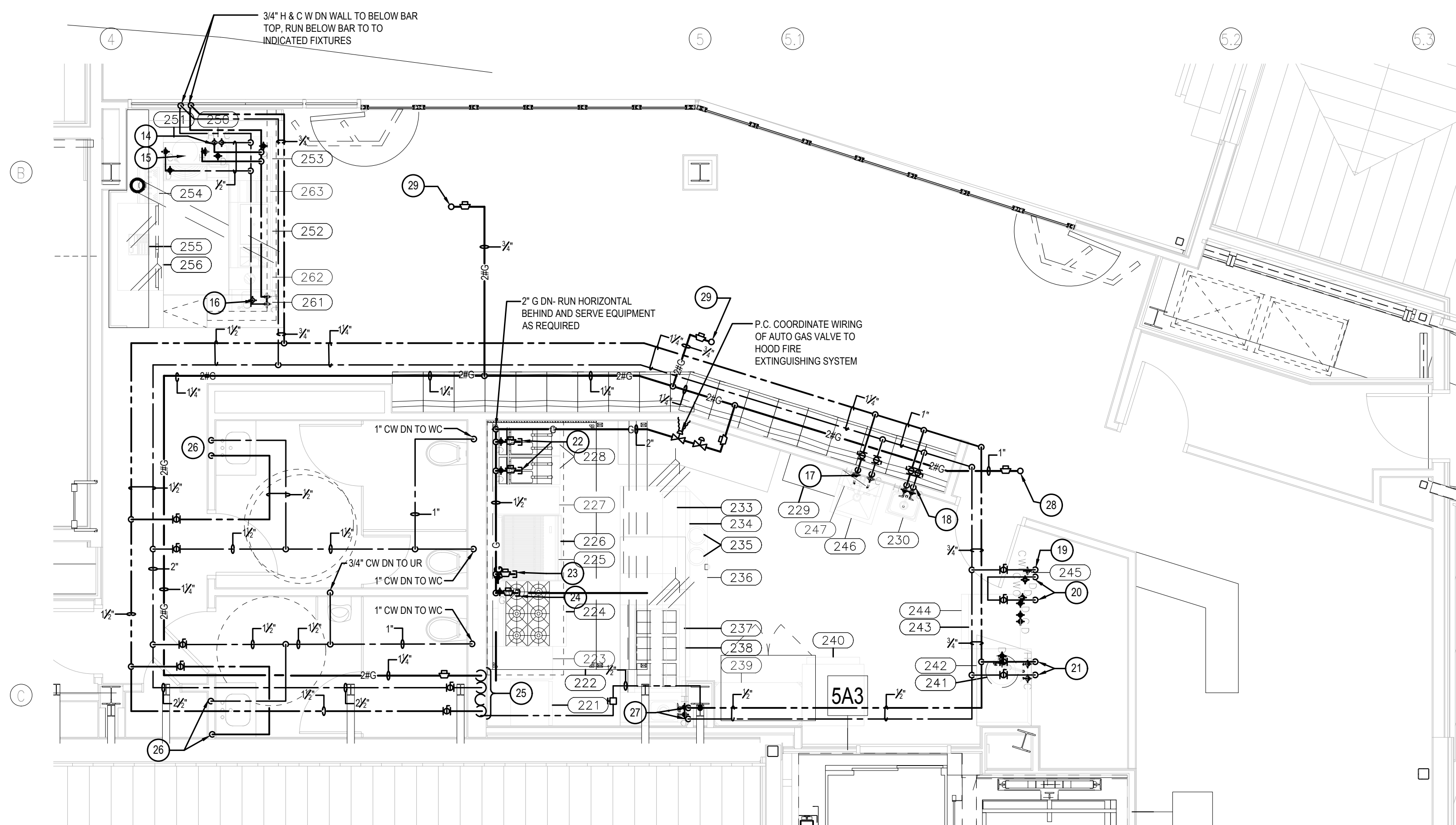
PENTHOUSE PLAN — DOMESTIC WATER PIPING WORK SCALE : 1/4" = 1'-0"
