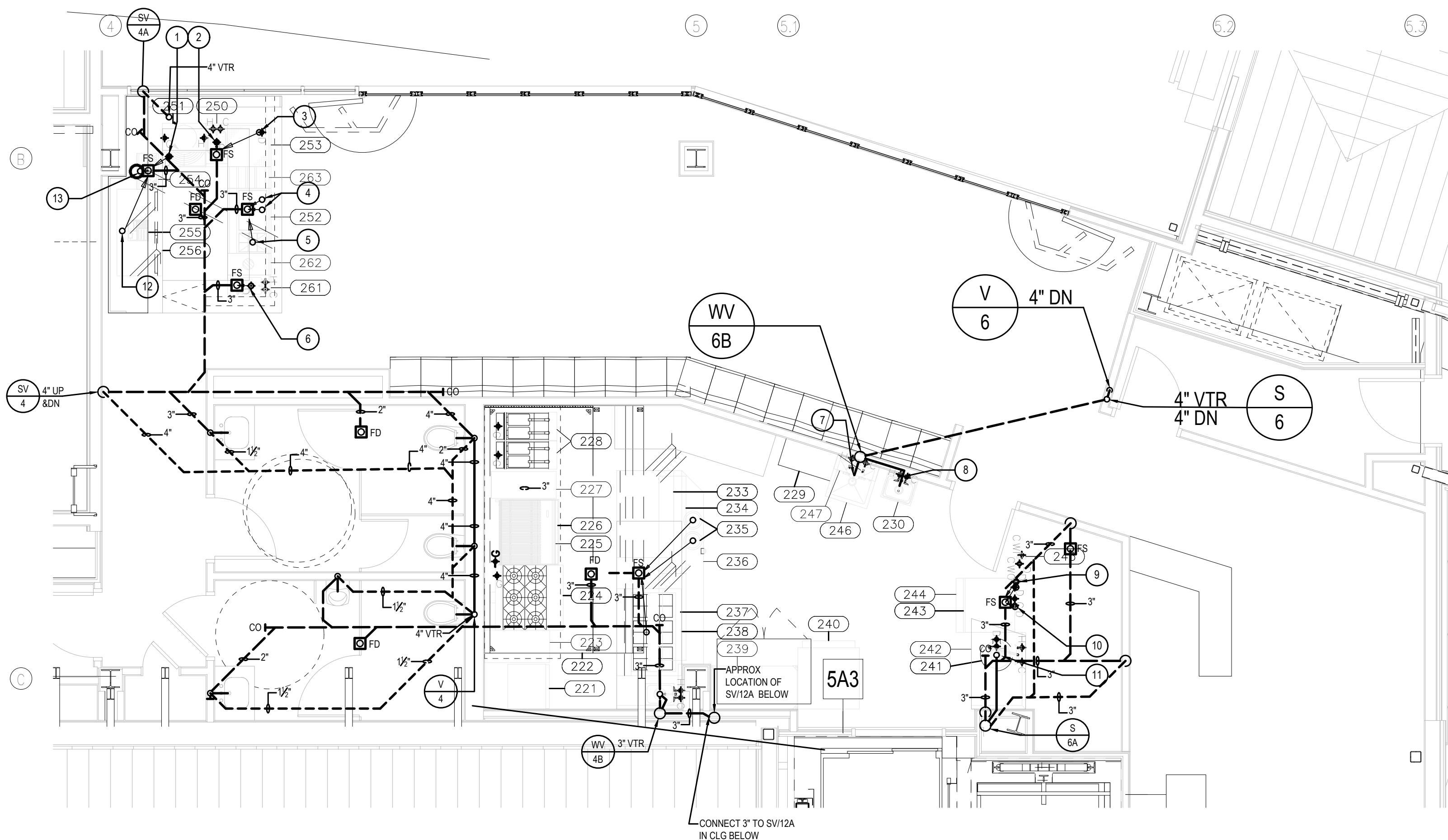
PENTHOUSE PLAN — SANITARY PIPING WORK SCALE : 1/4" = 1'-0"
