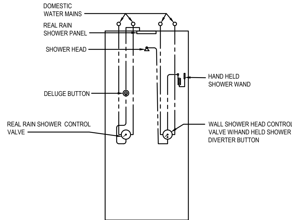
3 SHOWER WALL ELEVATION SCALE : NO SCALE
