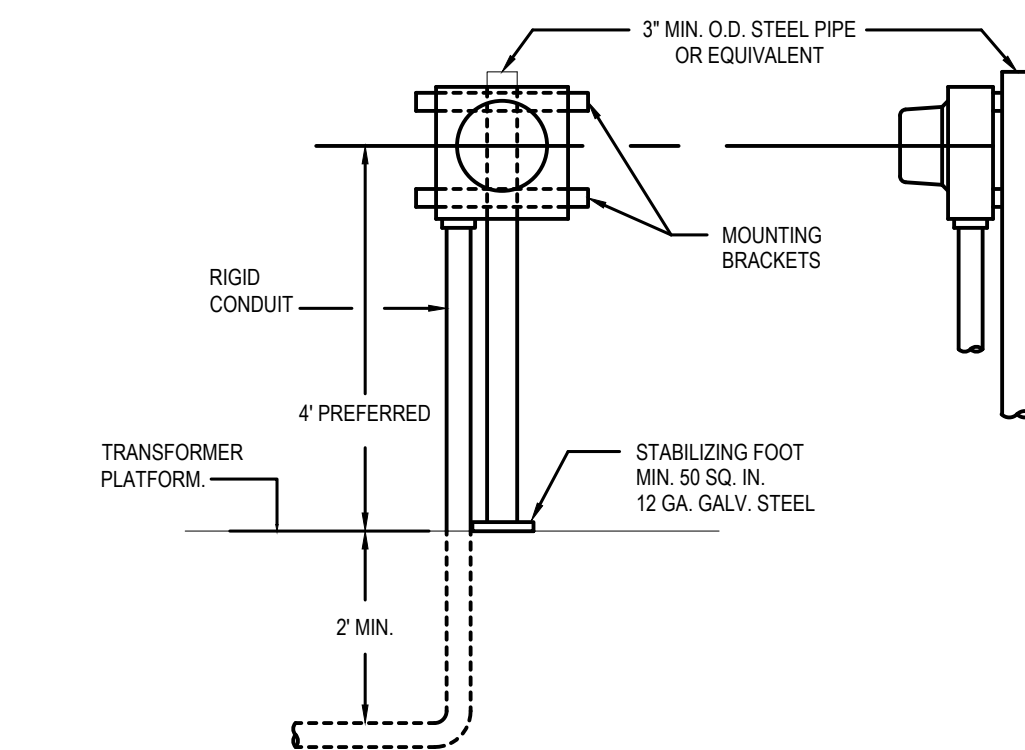
METER MOUNT DETAIL SCALE : NONE
