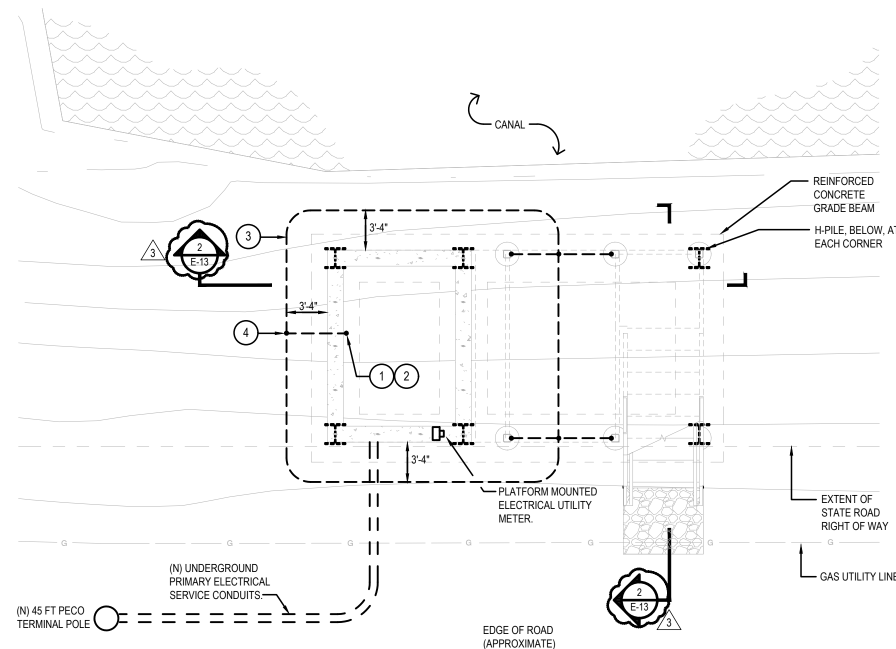
30" TRANSFORMER PLATFORM GROUNDING DETAIL PLAN SCALE : NONE
