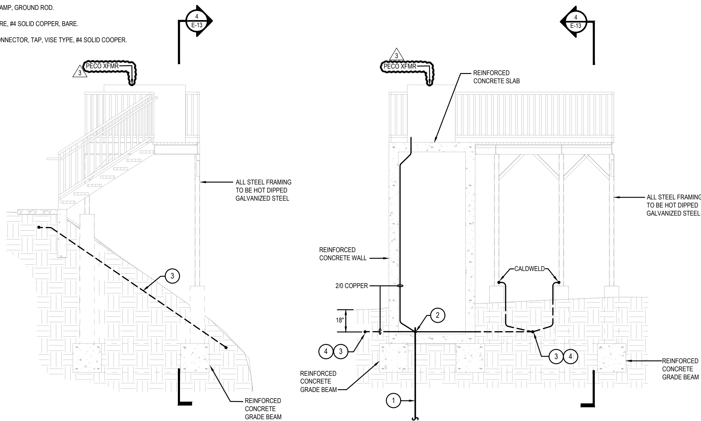
30" TRANSFORMER PLATFORM GROUNDING DETAIL SECTIONS SCALE : NONE
