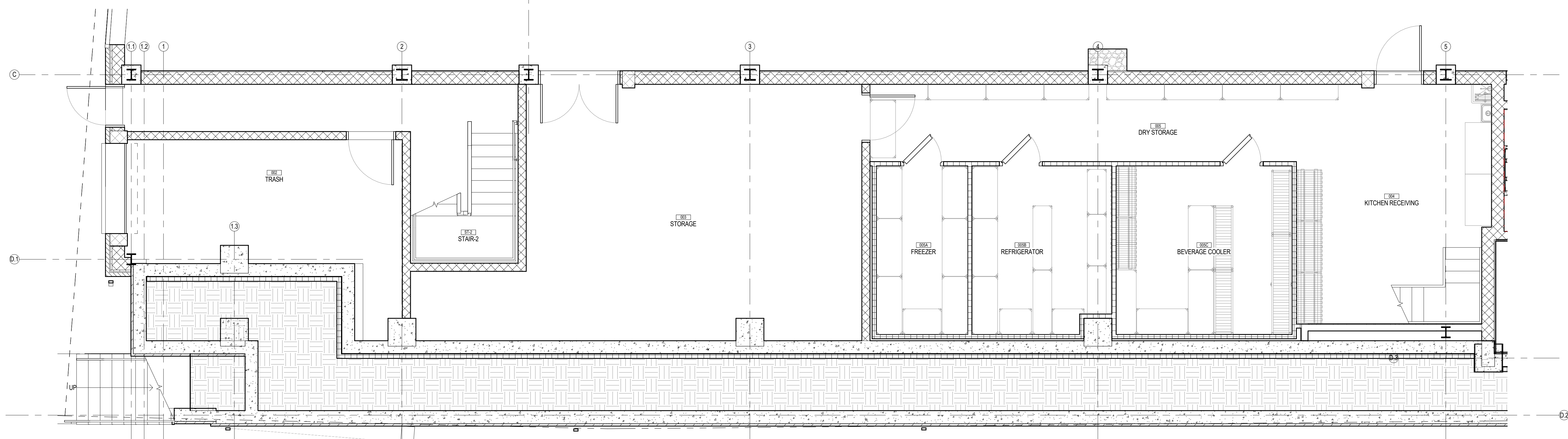
1 ENLARGED PLAN - 00 - KITCHEN STORAGE & RECEIVING A511 1/4" = 1'-0"
