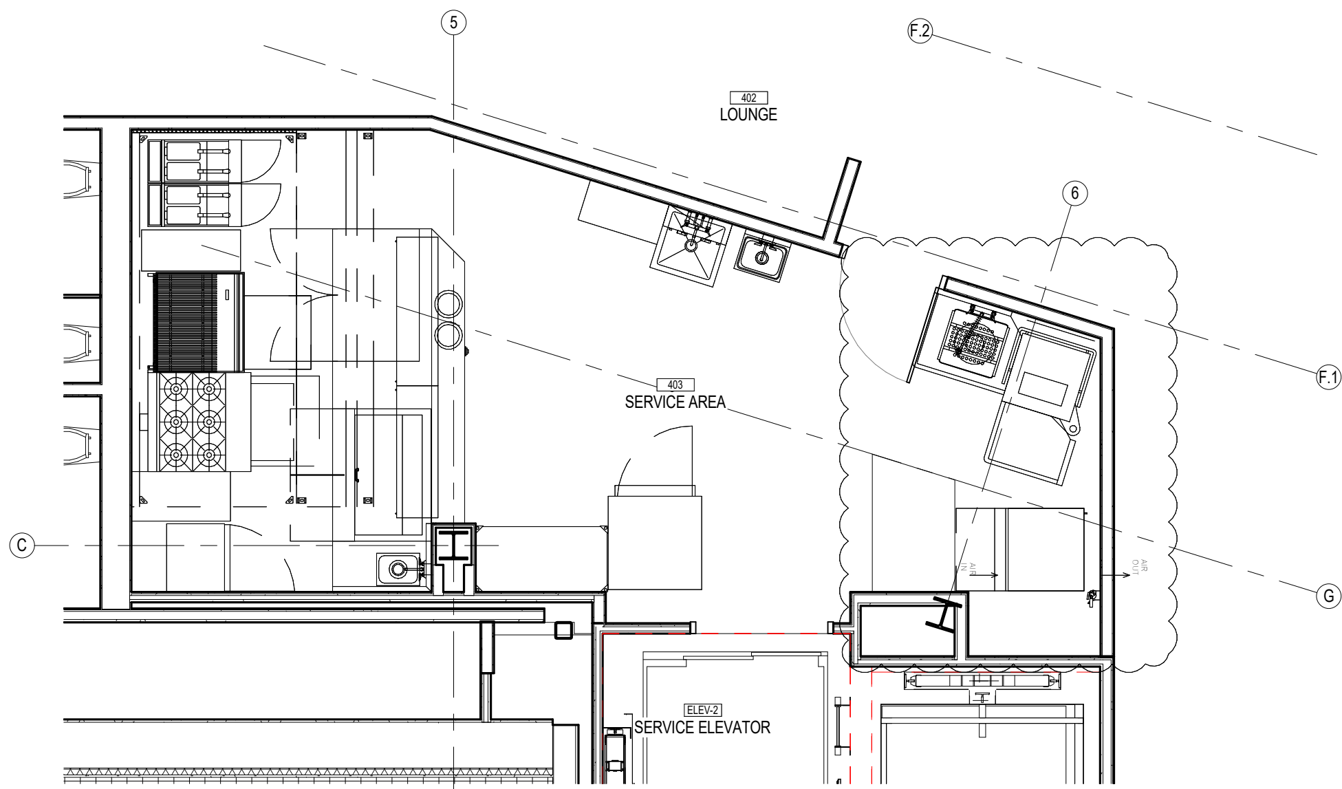
3 ENLARGED PLAN - 03 - PH KITCHEN A511 1/4" = 1'-0"
